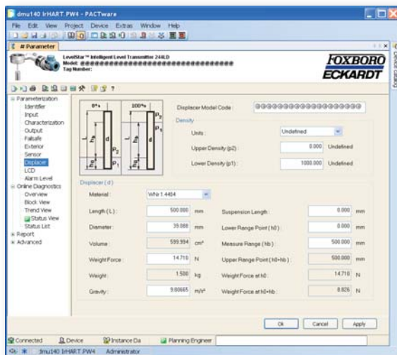
FDT-DTM: Configuration
